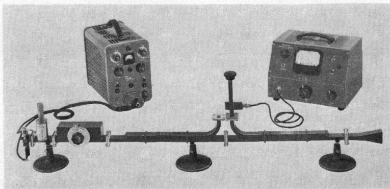
Fig. 1. Two -hp- multi-hole directional couplers in a reflectometer arrangement for measuring reflection coefficient magnitude. In background are an -hp- 715A klystron power supply to power signal source and an -hp- 415A standing-wave indicator to read output of detector.
