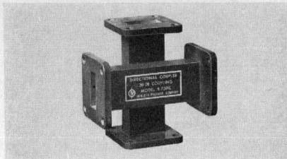
Fig. 6. -hp- Model 750 cross-guide type directional coupler.
